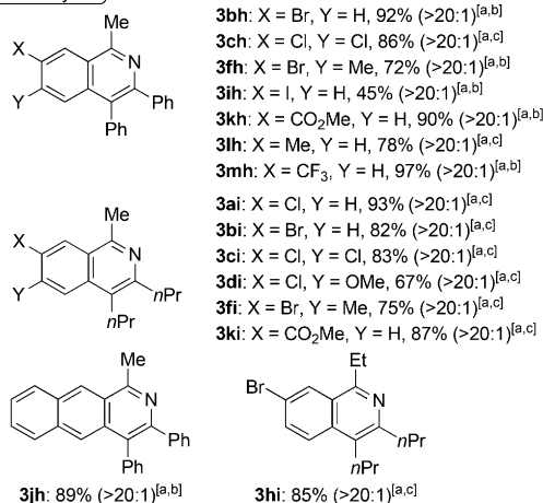
Scheme 2. Variation of unsymmetrical O -acyl oximes 1 . Reaction conditions: 1 (0.15 mmol), 2 (0.18 mmol), [Cp*Co(CO)I 2 ] (10 mol%), AgSbF 6 (20 mol%), and KOAc (20 mol%) in ClCH 2 CH 2 Cl at 120 °C for 24 h unless otherwise noted. Combined yields of isolated 3 and its regioisomer 4 are given. The numbers in parentheses correspond to the ratios of 3/4 determined by 1 H NMR analysis of the crude mixture. [a] CsOAc (20 mol%) instead of KOAc. 1 (0.10 mmol) and 2 (0.15 mmol) were used. [b] 80 °C. [c] 100 °C. Cy = cyclohexyl.
