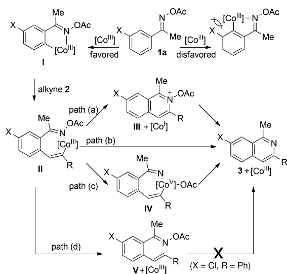
Figure 1. Possible reaction pathways for the formation of isoquinolines under \text{Cp}^*\text{Co}^{\text{III}} catalysis.
