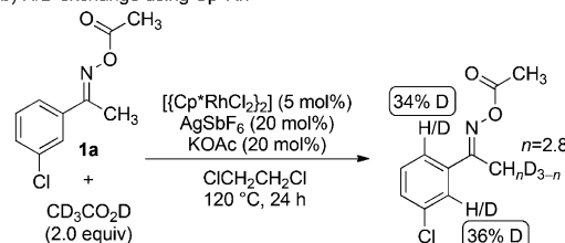
Scheme 4. H/D exchange experiments under a) Cp*Co III catalysis and b) Cp*Rh III catalysis.
