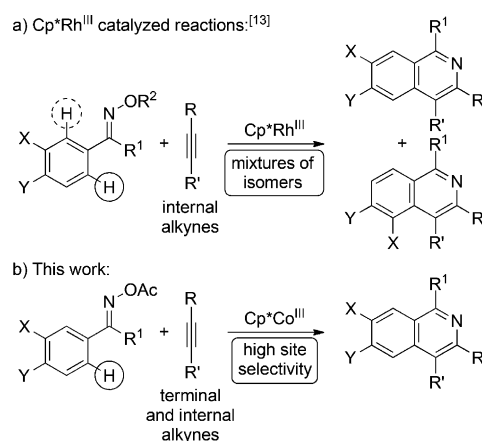
Scheme 1. Cp*Rh III and Cp*Co III catalyzed isoquinoline syntheses; site selectivity with unsymmetrical oxime derivatives and alkynes.
